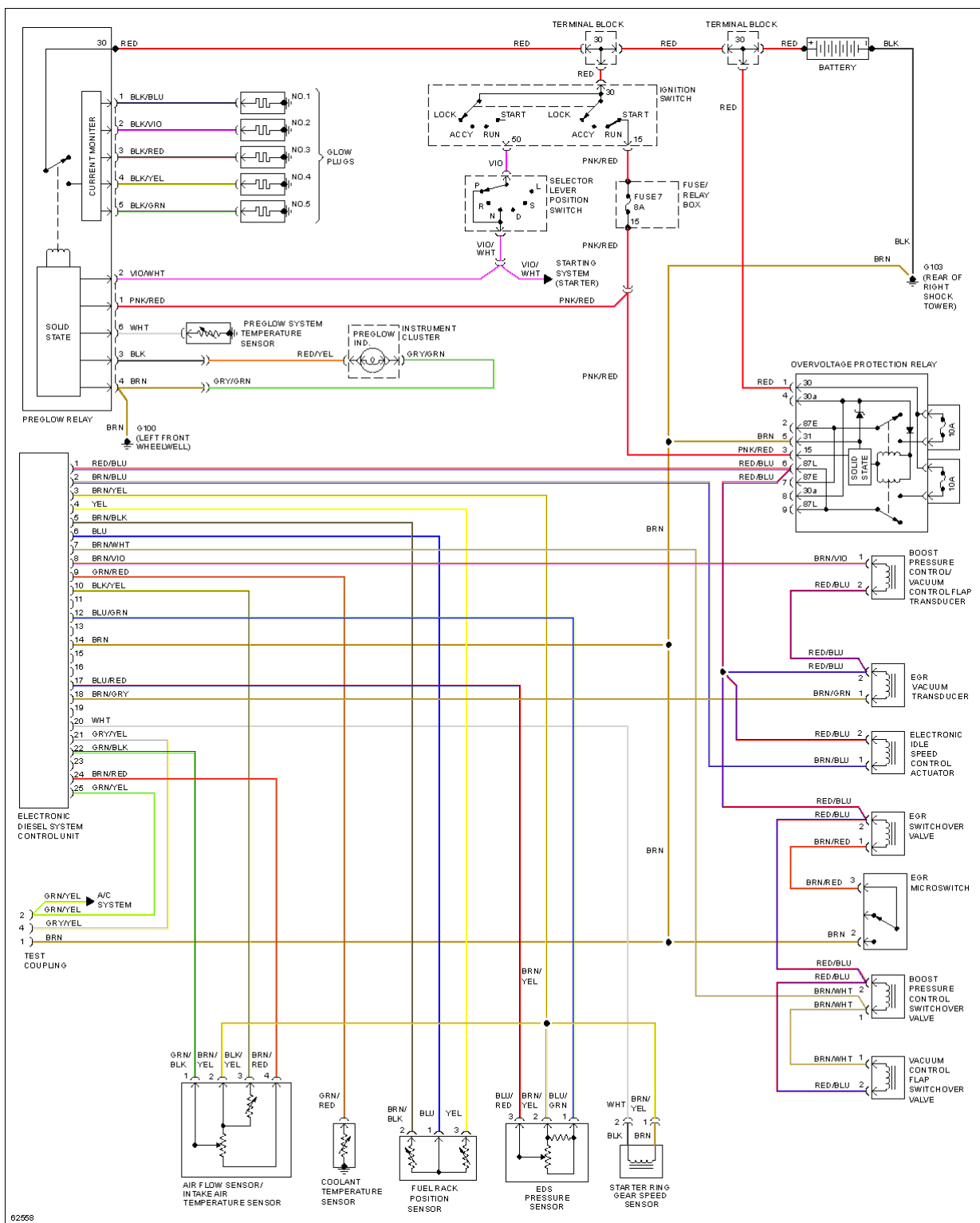
Fig. 7: 2.5L Turbo Diesel, Engine Performance Circuits
