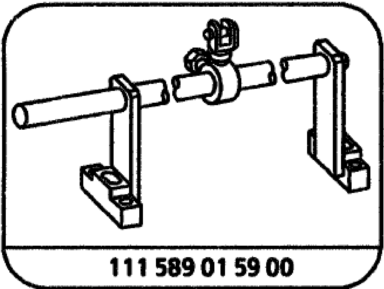
Supporting Beam
