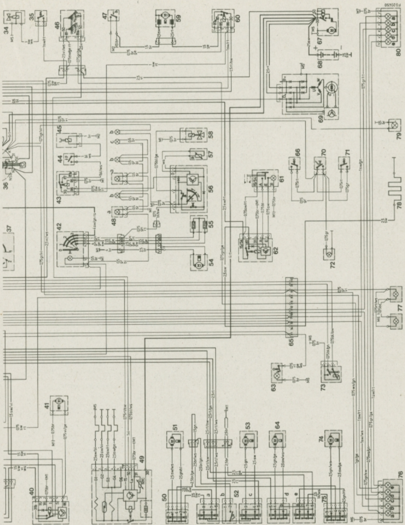
1981 240D (123.123 US) wiring diagram
