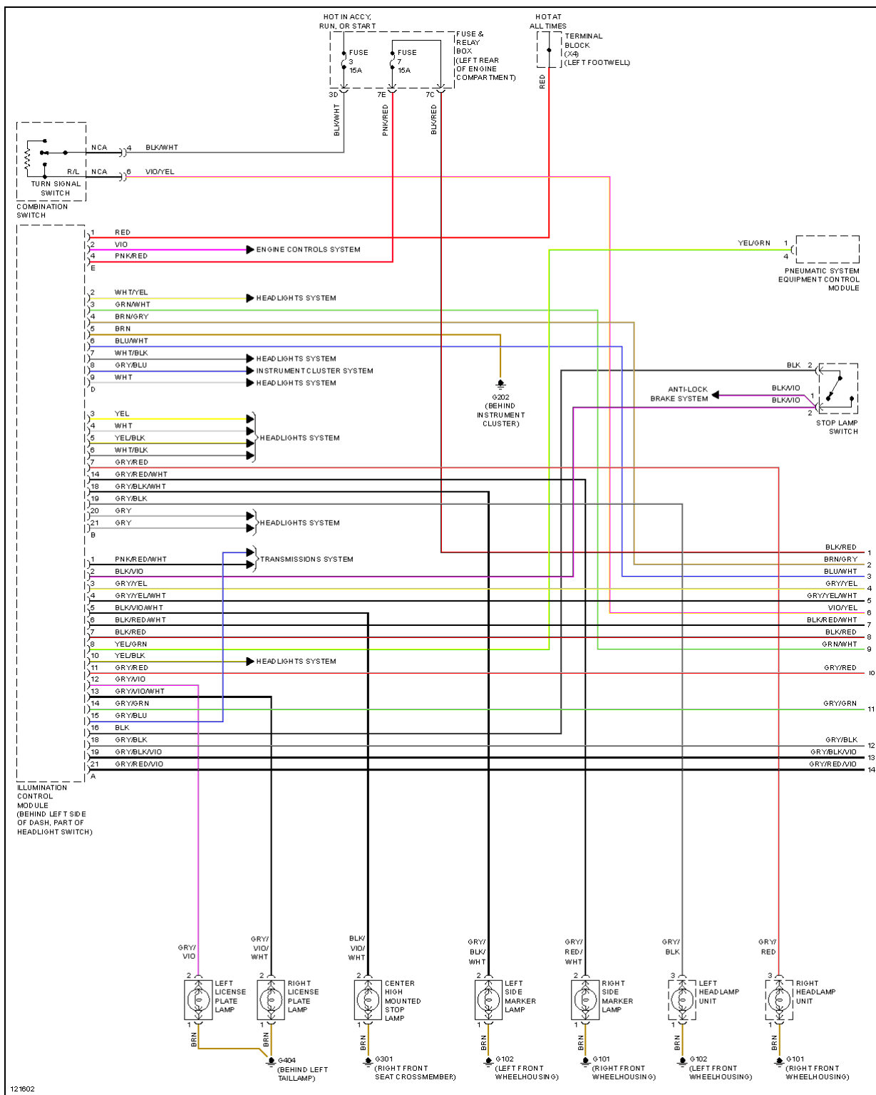
Fig. 14: Exterior Light Circuit (1 of 2)
