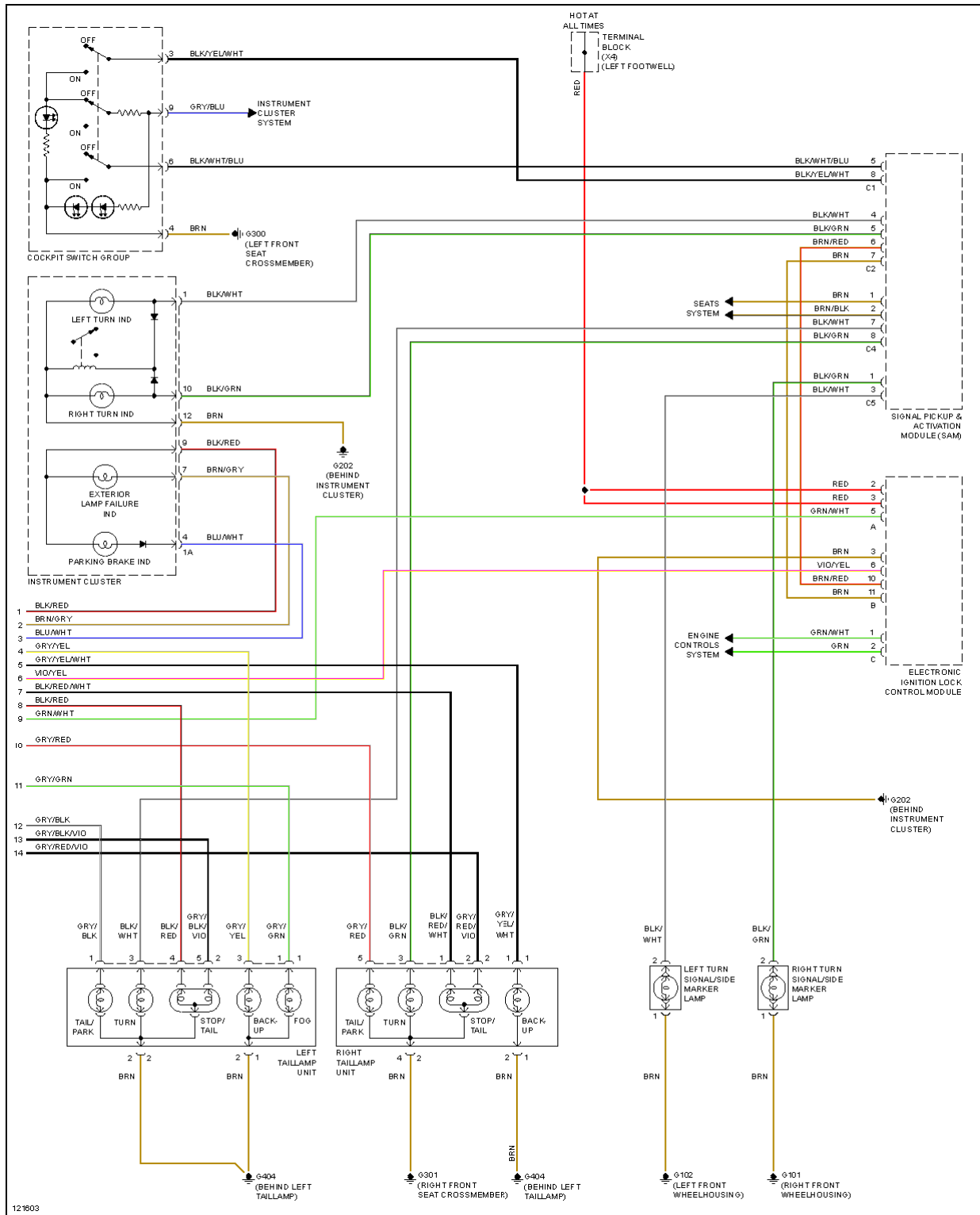
Fig. 15: Exterior Light Circuit (2 of 2)
