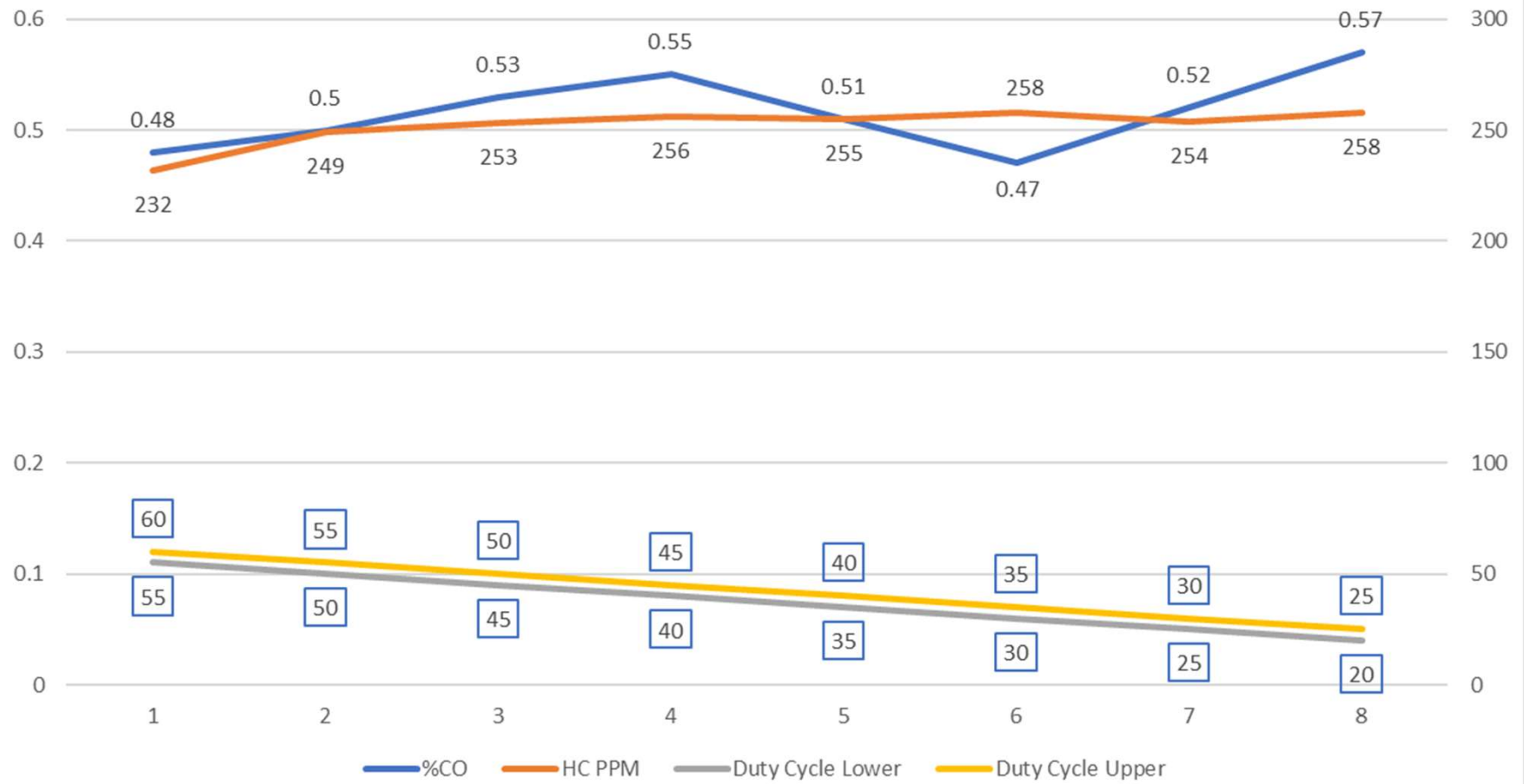
%CO and HC PPM vs Duty Cycle 1990 Mercedes 300 SEL
