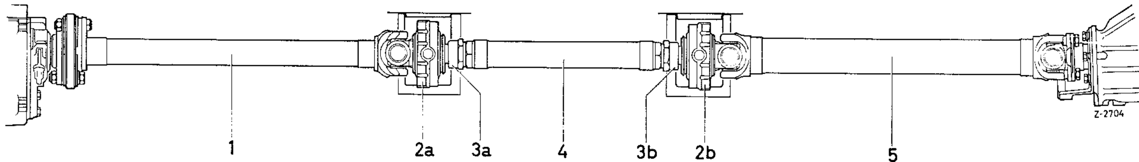
Fig. 41-1/2 3-part universal shaft
