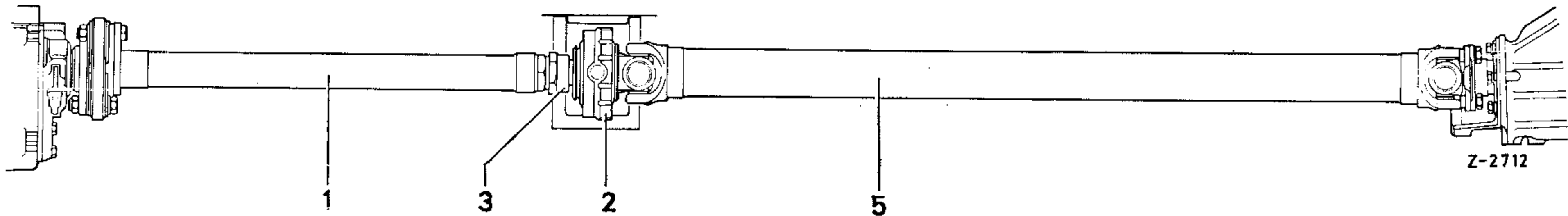
Fig. 41-1/1 2-part universal shaft
